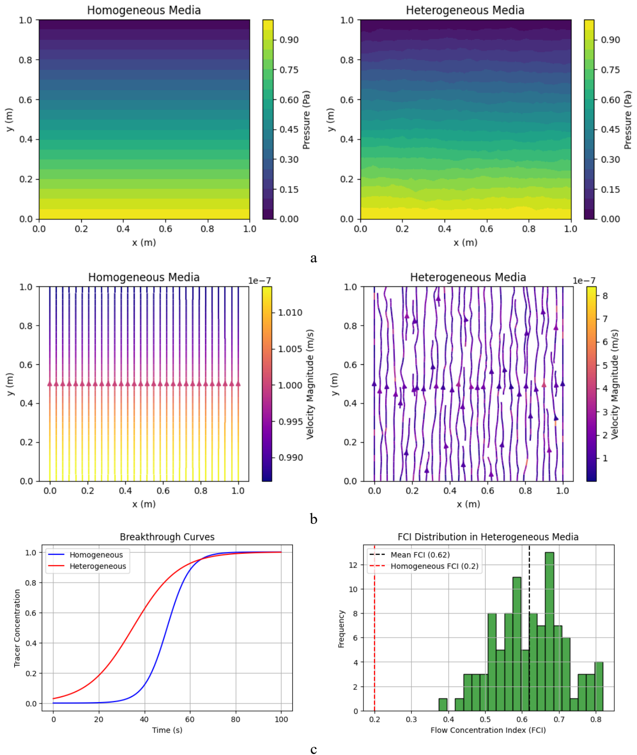
a – distribution of pressure; b – velocity fields of the flow; c – flow concentrations
